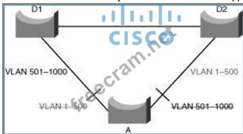
Figure 3-15: VLAN Load Balancing
